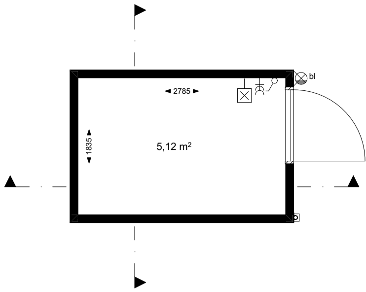
00 Begane grond 1:50
